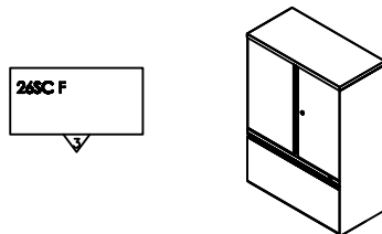
S5- 1 File Drawer with 26h Storage Case Unit 30w 15d 42h - Laminate
